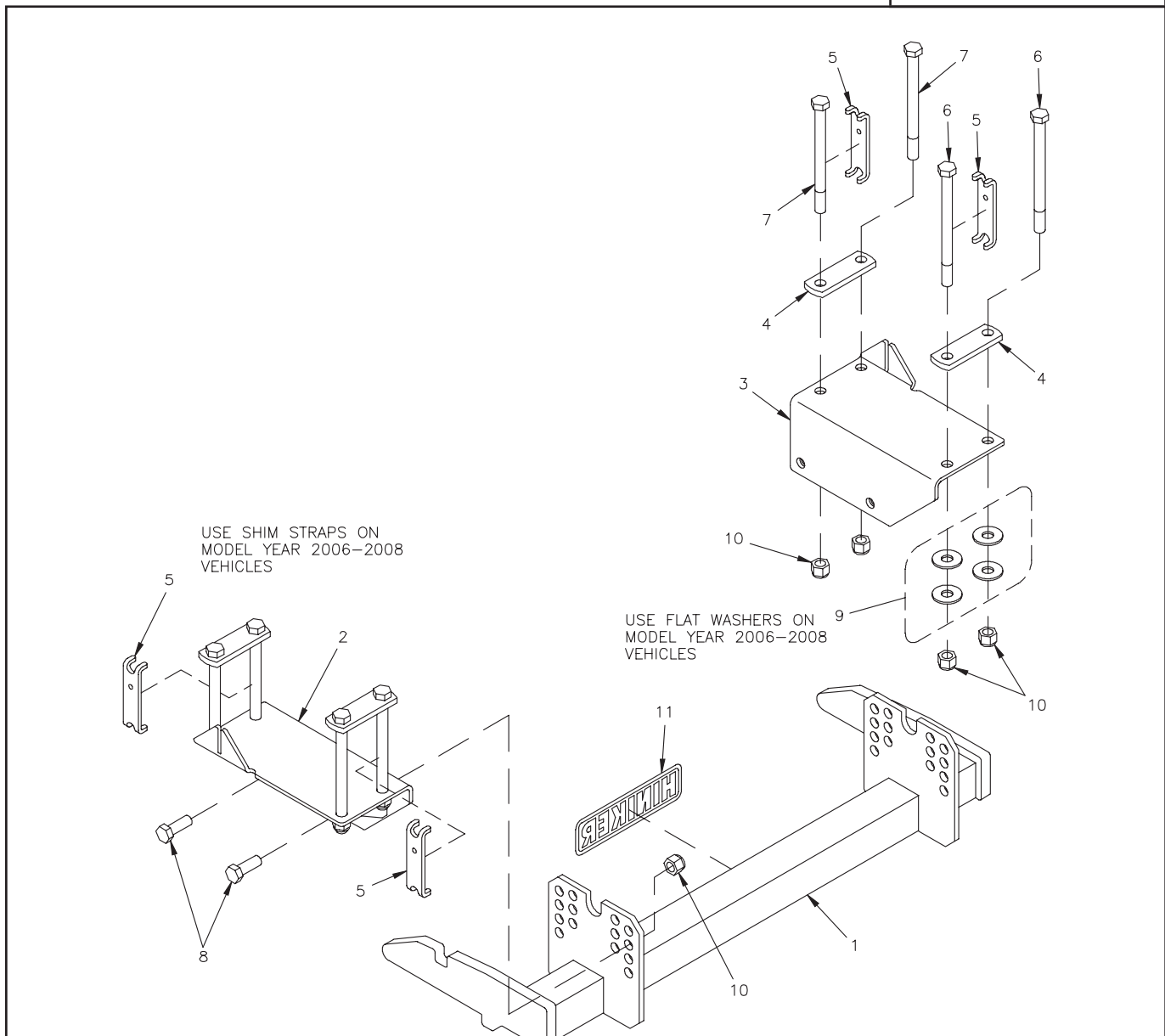
25011815 Mount Kit
