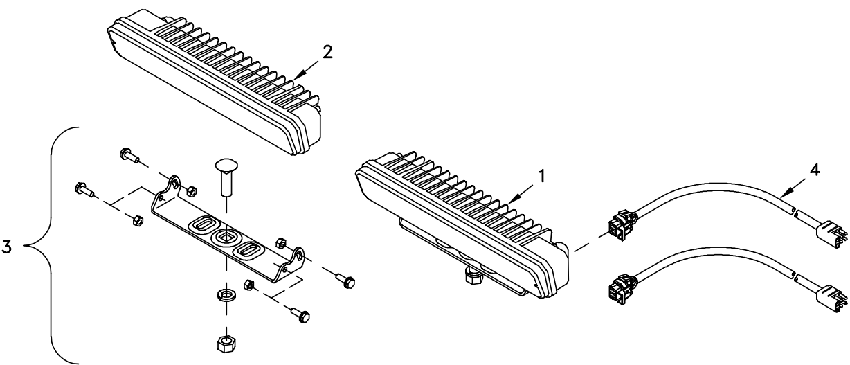
25014159 LED Headlight Pair (Items 1, 2, 3) DWG. NO. 7810
