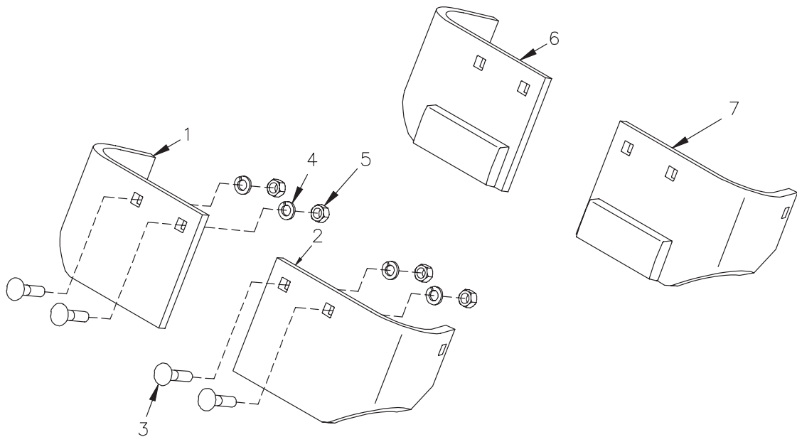
25011695 Curb Guard Kit - Standard 25012726 Curb Guard Kit With Wear Bars DWG. NO. 5486
