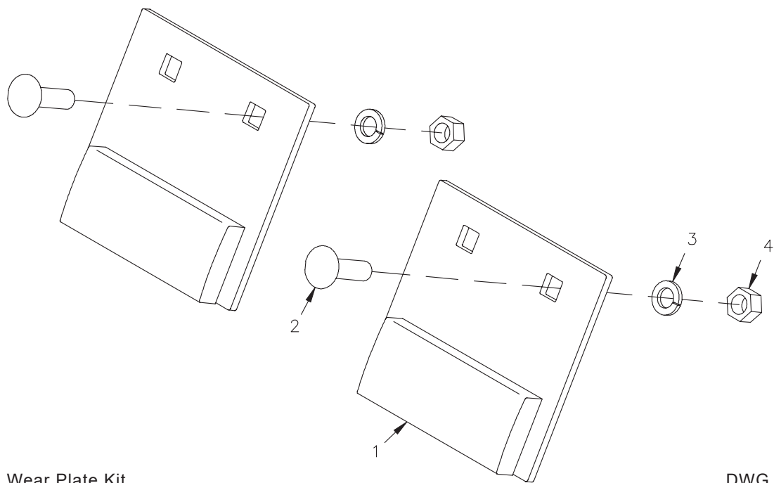
25012587 Wear Plate Kit DWG. NO. 6331
