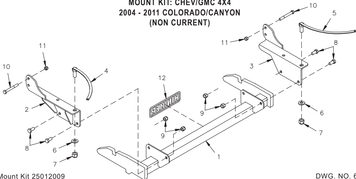
Mount Kit 25012009
