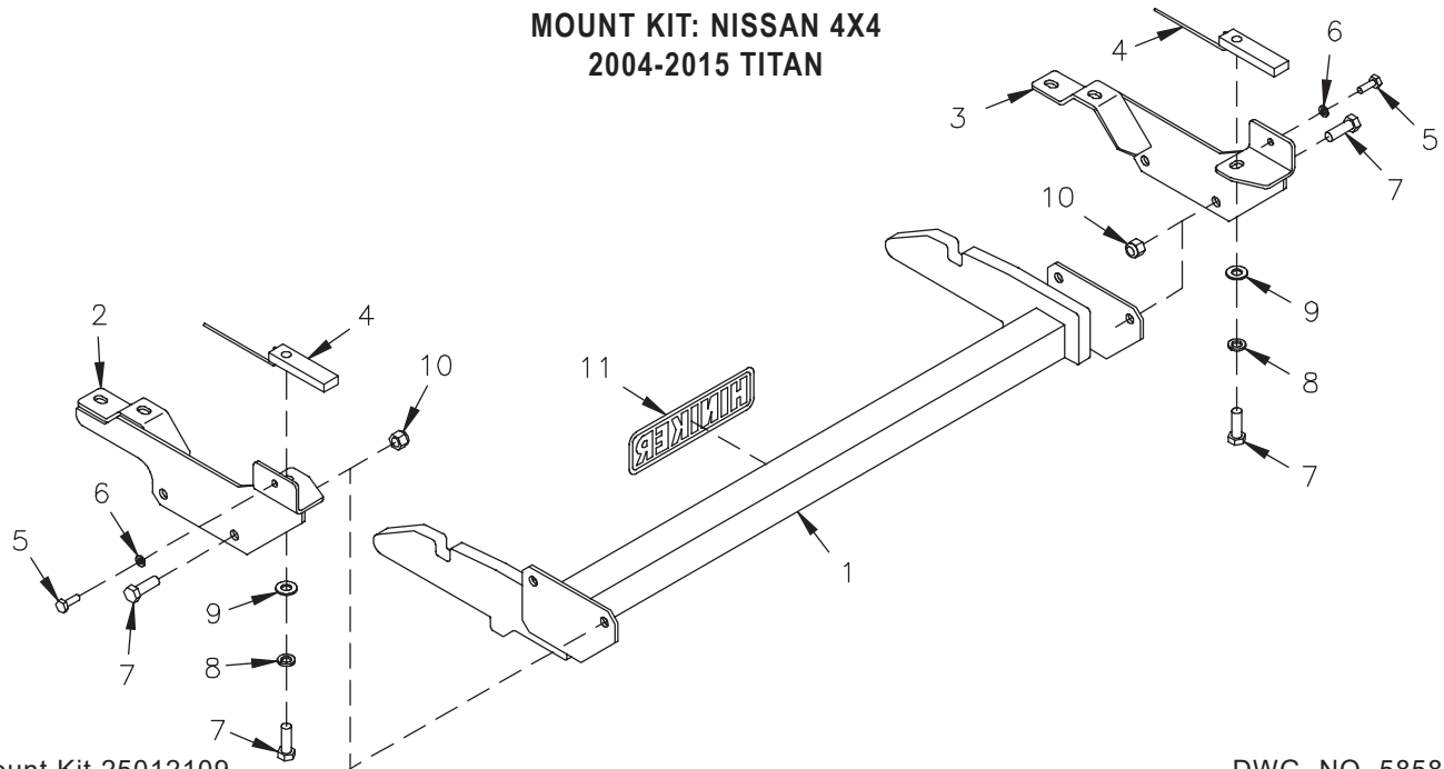
Mount Kit 25012109
