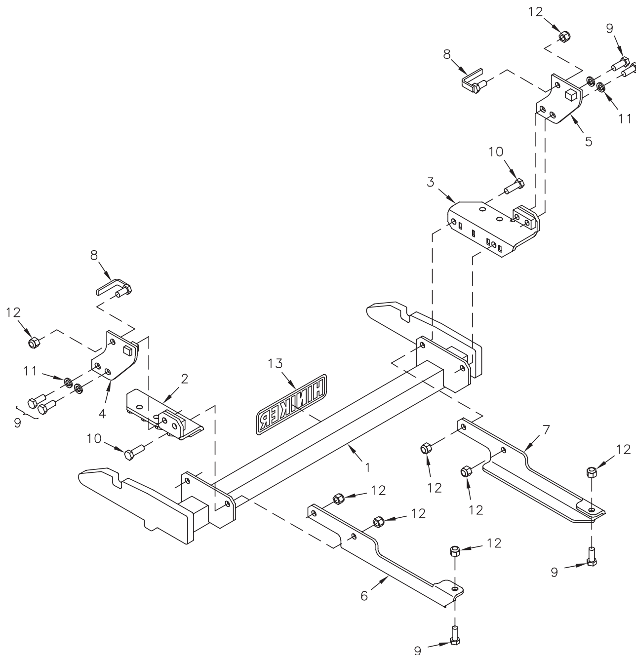
Mount Kit 25012508
