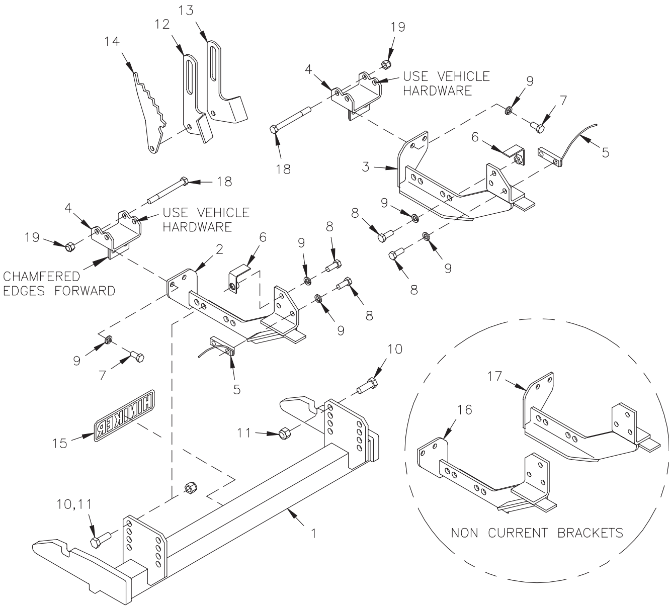
Mount Kit 25013567
