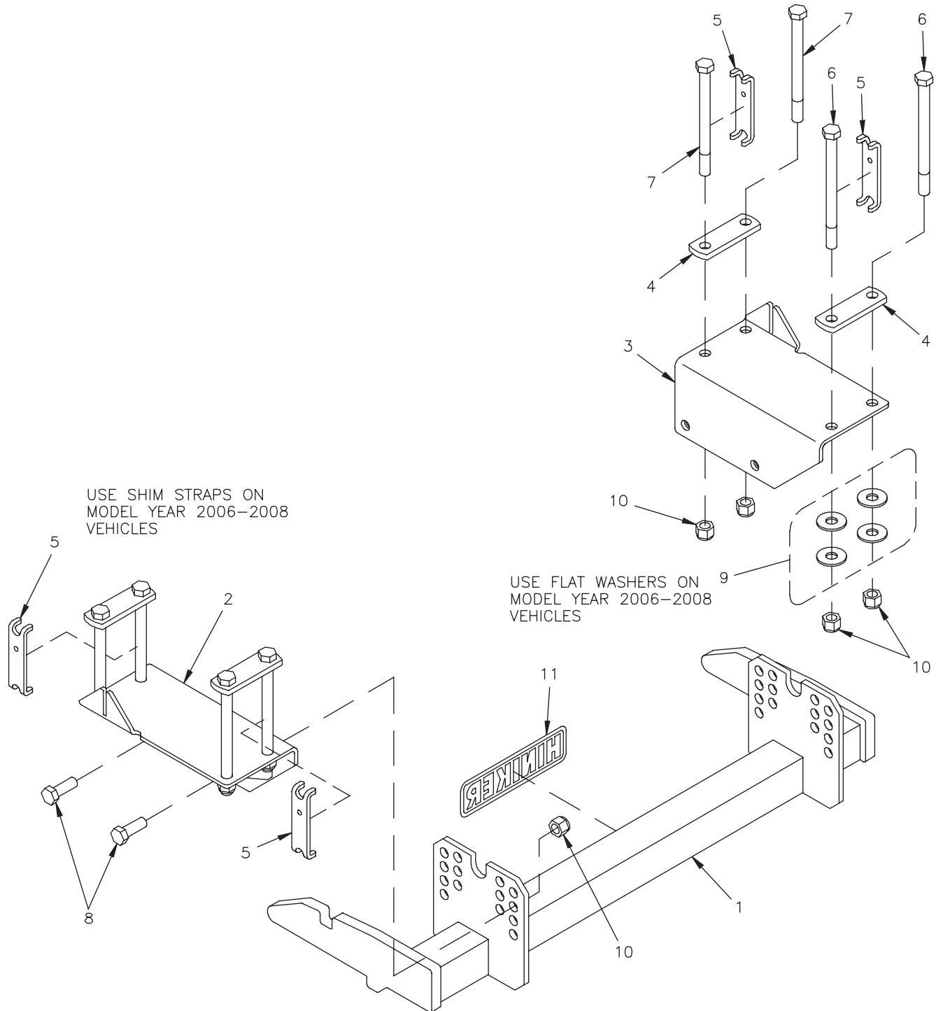
Mount Kit 25011815
