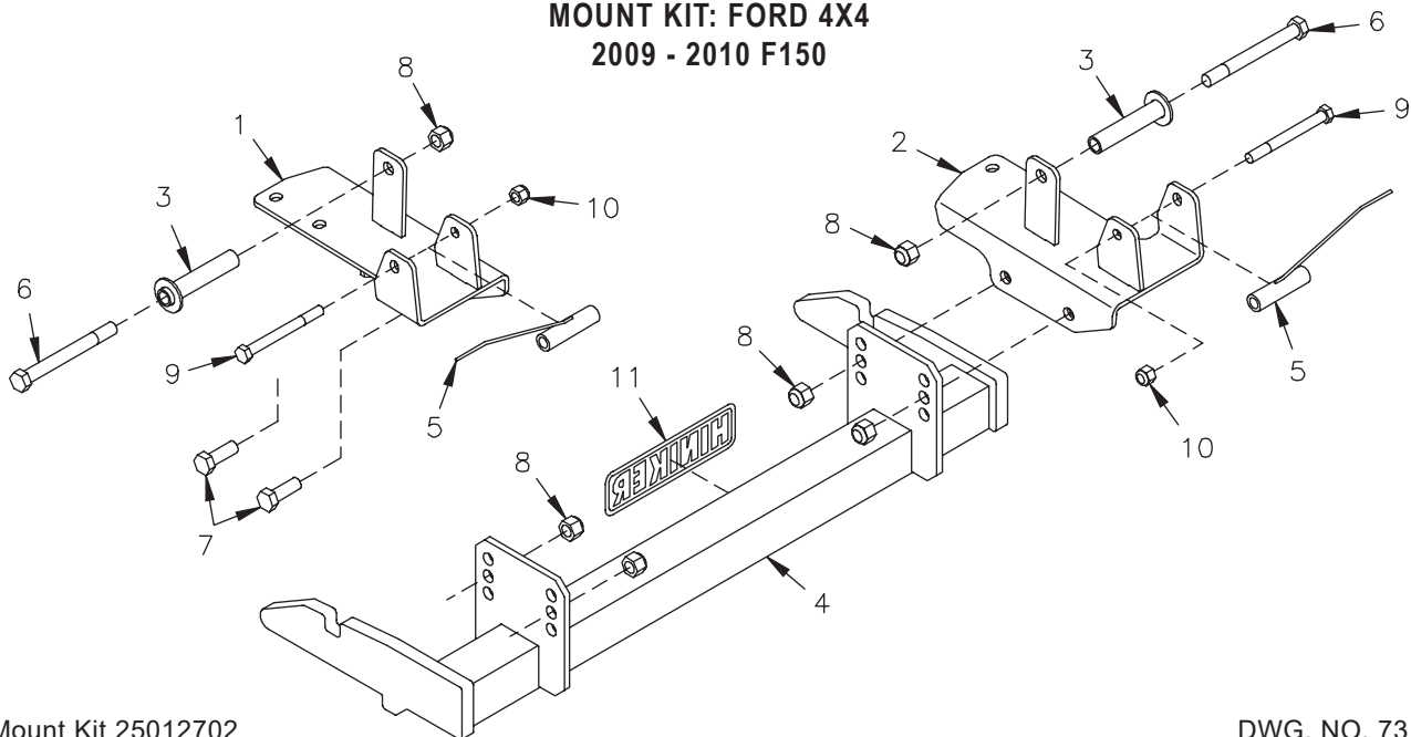
Mount Kit 25012702
