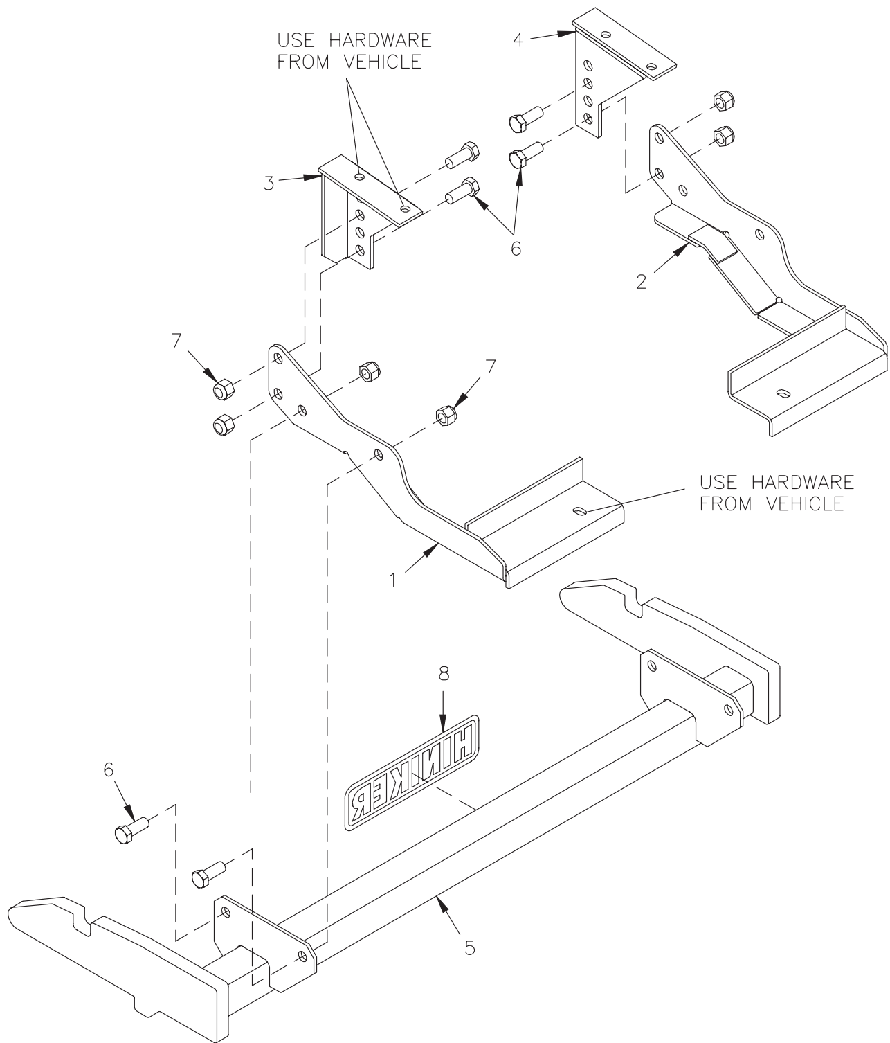
Mount Kit 25012022
