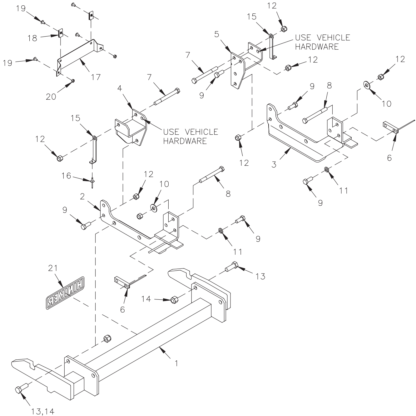
Mount Kit 25012206
