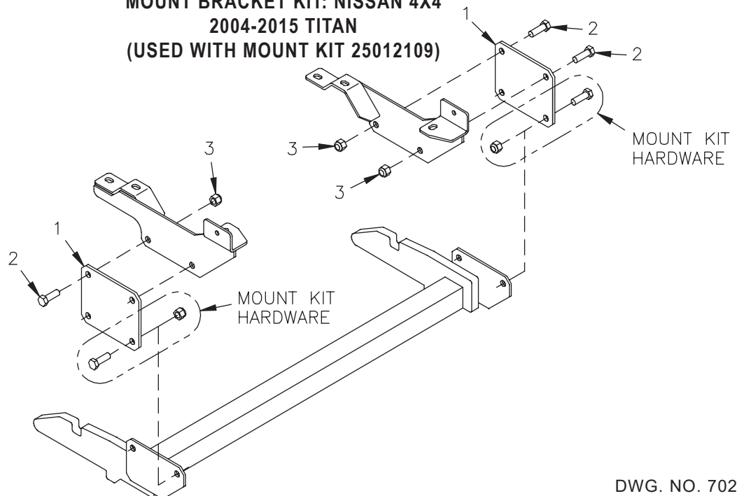
Adapter Kit 25013346
