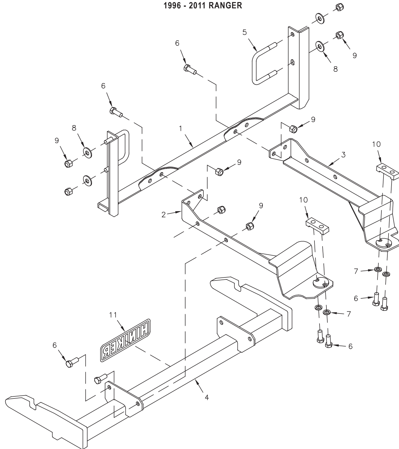
Mount Kit 25012024
