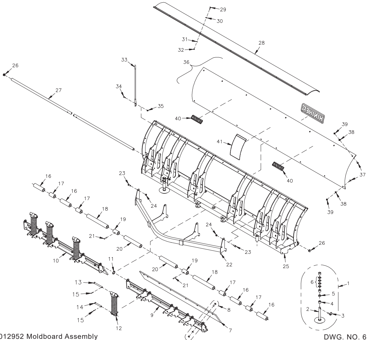
25012952 Moldboard Assembly
