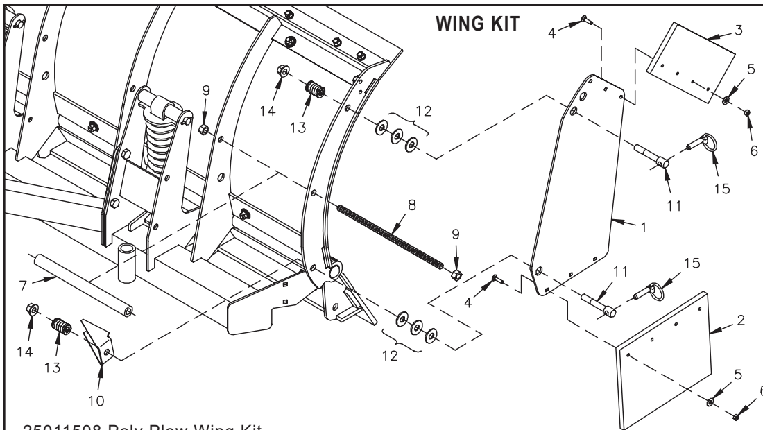
25011508 Poly Plow Wing Kit
