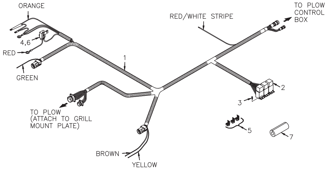
DWG. NO. 3943A
